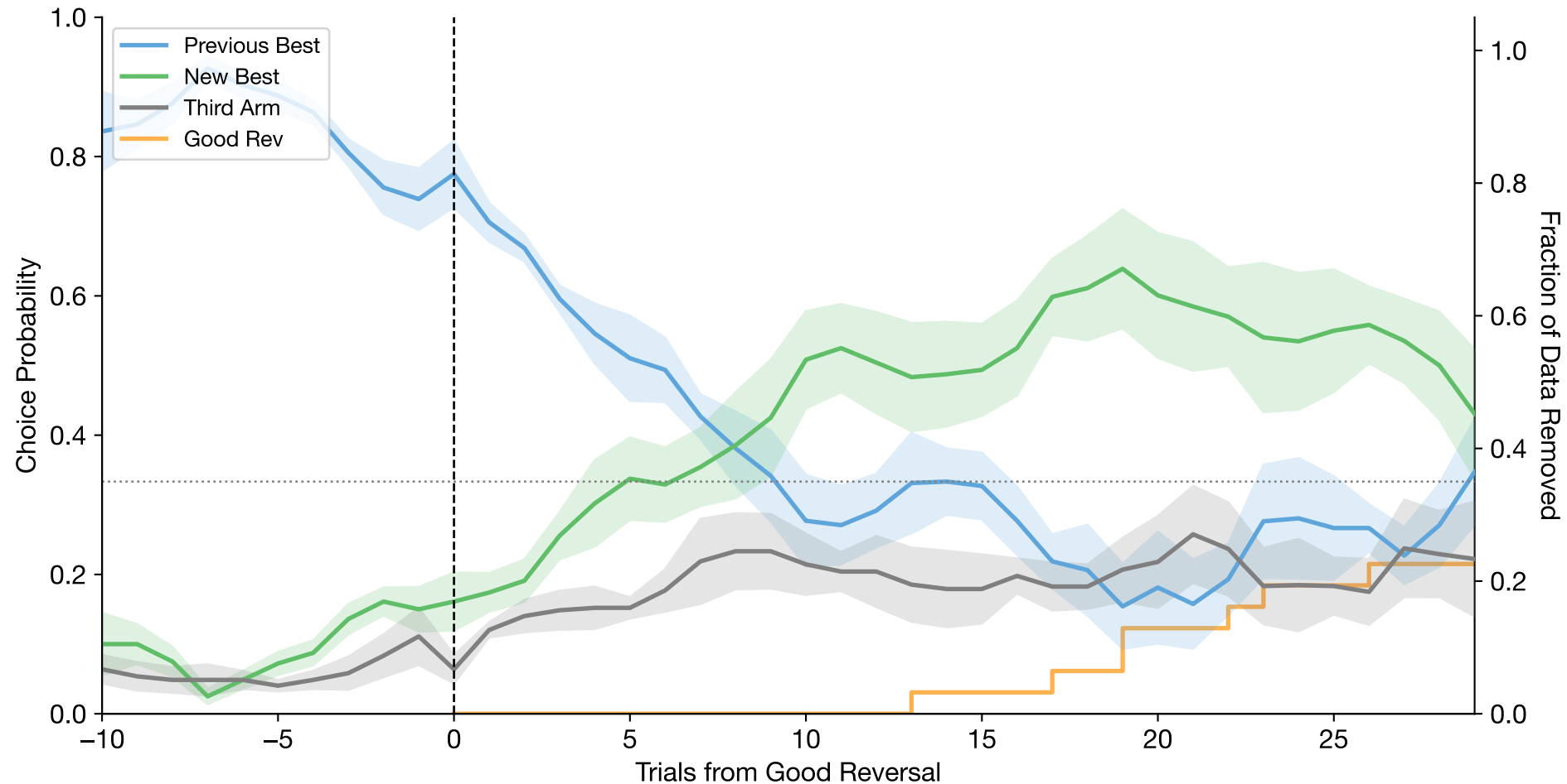
Good Reversal-Aligned Choices (mean \pm se across subjects | n=6 subjects, n=31 reversals)
